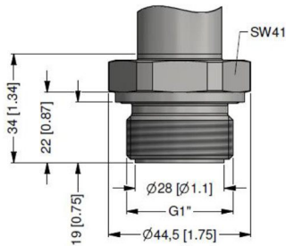
G1" flush
