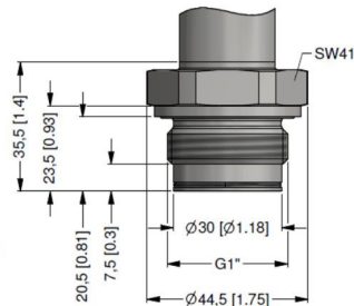
G1" flush with radial o-ring ( P_N > 0.25 bar)
