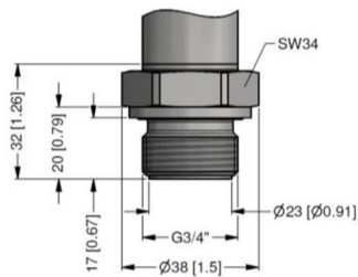
G3/4" flush
