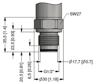
G1/2" flush with radial o-ring
