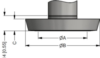
dairy pipe (DIN 11851)
