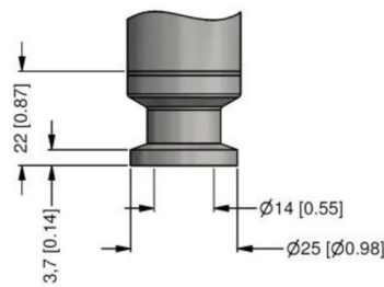
Clamp 3/4" (DIN 32676) 4 bar \leq P_N \leq 8 bar
