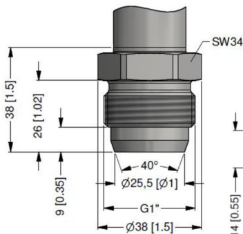
G1" cone
