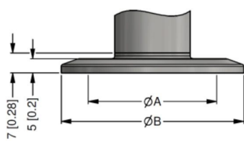
clamp (DIN 32676)
