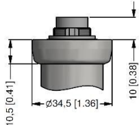
Binder Series 723 5-pin (IP 67)
