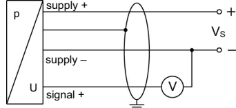
3-wire-system (voltage)
