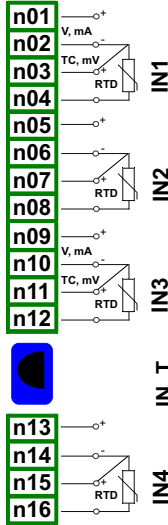
QFUN4 4 universal inputs
