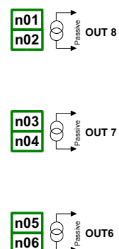
IO8 8 current outputs
