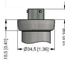
Binder Series 723 7-pin (IP 67)
