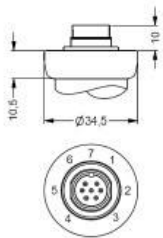
Binder series 723 7-pin (IP 67)
