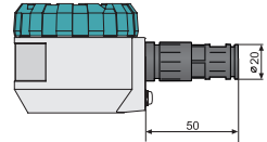
Variant CLM-70 with a cable gland for protective hose H1
