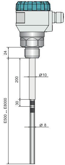
Variant CLM-70 with a cable gland for protective hose H1
